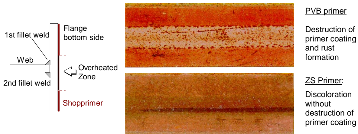
Figure1: Corrosion at the bottom side of the double fillet weld samples after one-month outdoor storage
