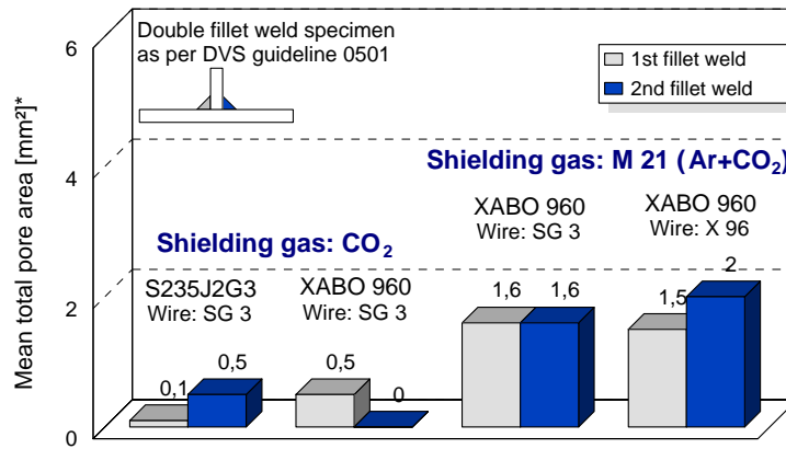
Figure 3: Influence of shielding gas, base metal and filler metal on the tendency to pore formation when welding through the zinc silicate shop primer 1589
