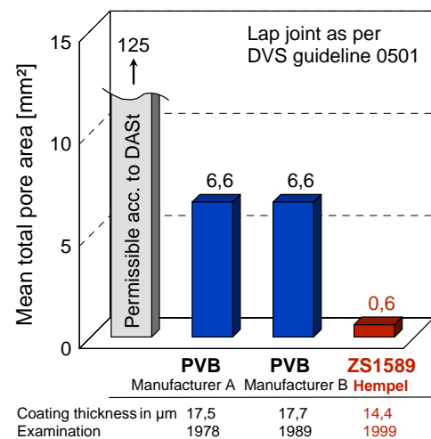
Figure 4: Investigations of the SLV Duisburg
