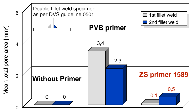
Figure 2: Comparison of PVB and zinc silicate shop primers (base metal: S235J2G3, wire electrode: SG 3, shielding gas: CO 2 )
